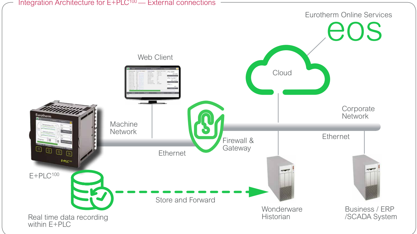
Integration Architecture for E+PLC 100 — External connections
